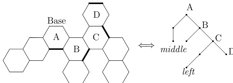
Figure 1: Benzene Molecules and the corresponding HR -tree.
