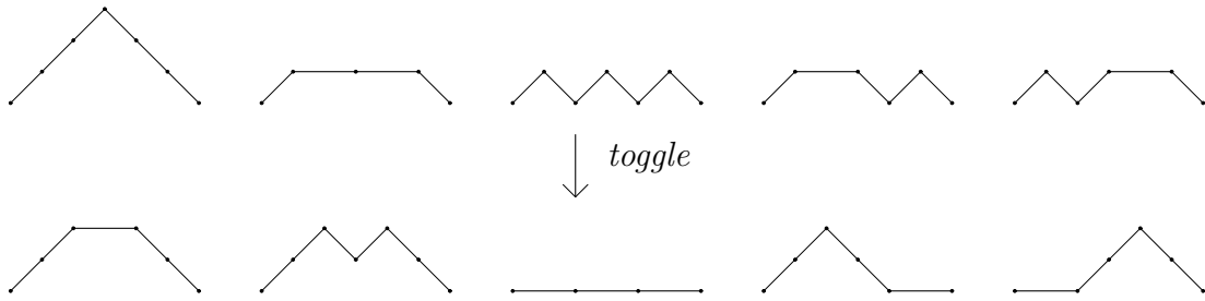
Figure 3: (Catalan) Schröder paths of length 6.
