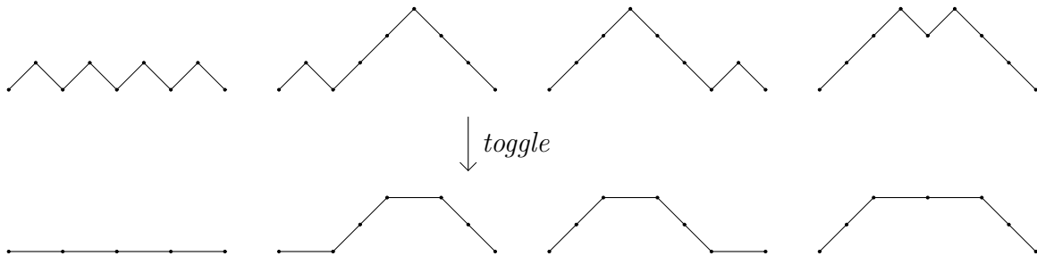
Figure 5: (Motzkin) Schröder paths of length 8.
