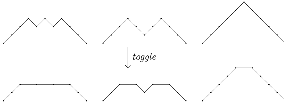
Figure 6: (Riordan) Schröder paths of length 10.
