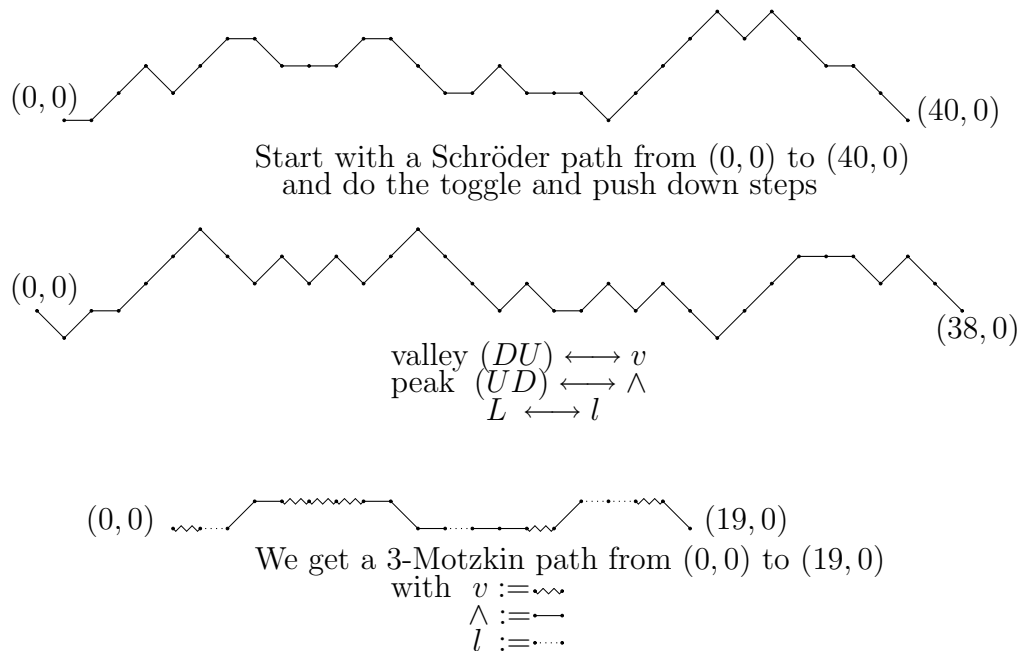
Figure 2: The bijection \phi
