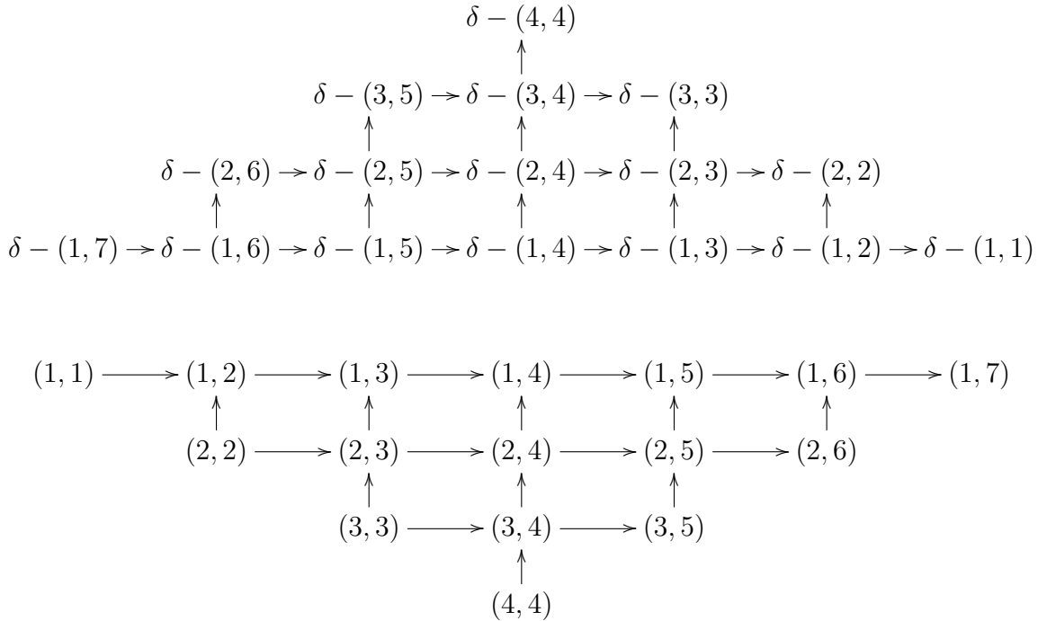
Figure 5: D_2 and D_3
