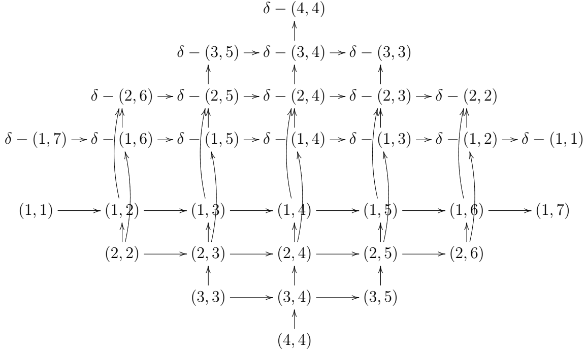
Figure 6: Completed \tilde{B}_4 diagram
