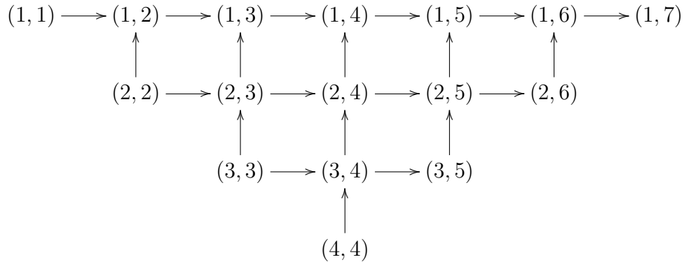
Figure 1: Positive roots in B_4
