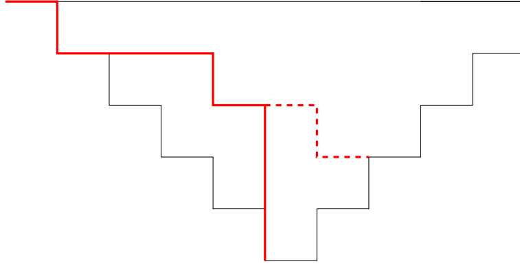
Figure 9: Modication of the Dyck path rfrrrfrfff
