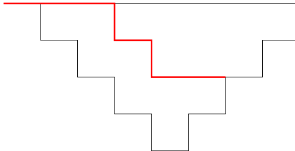
Figure 3: An example of the B_4 -path rrrfrfrr
