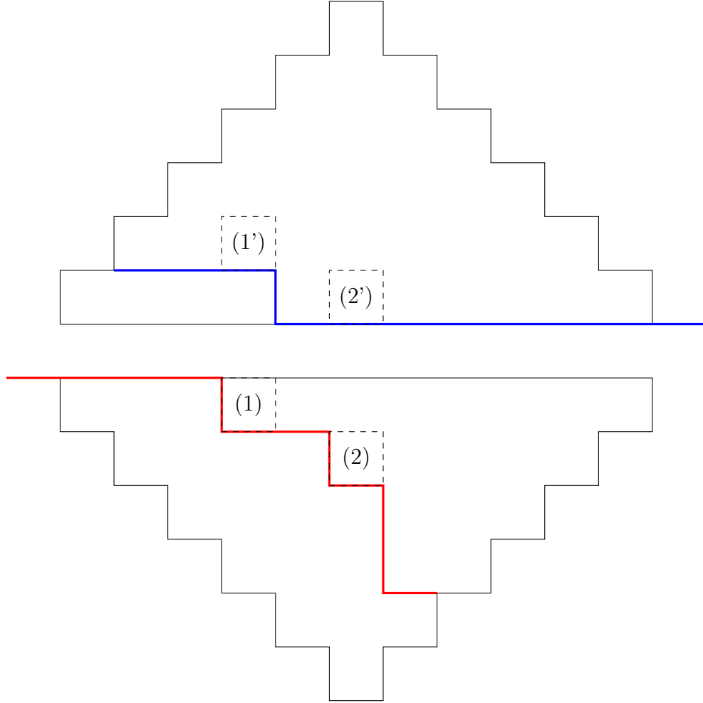
Figure 8: A pair of paths
