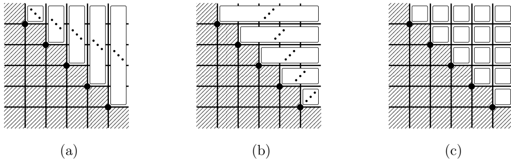
Figure 2: The structure of \text{Av}_n(p, r) from Proposition 13
