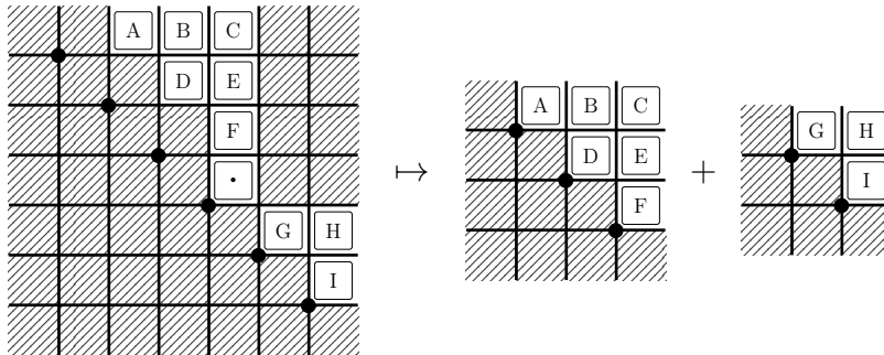
Figure 5: Decomposing a permutation in Av_n(p, r) from Proposition 18
