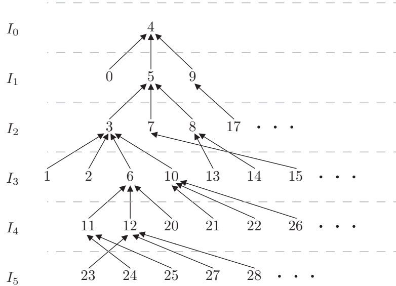
Figure 1: A partial digraph representation of the first six iterated sets of \mathcal{W} .
