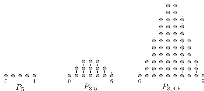
FIGURE 1. The tiles P_5 , P_{3,5} and P_{3,4,5} . The multiplicity with which an integer appears inside the tile is indicated by the number of points in the column above it.
