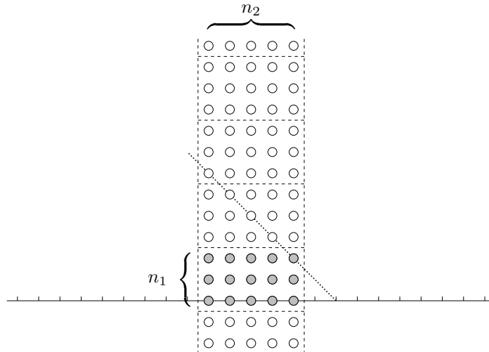
FIGURE 4. A coordinate-sum representation of a P_{n_1, n_2} -tiling of level n_2 .
