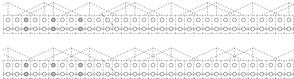
FIGURE 8. More P_{3,2}^{3,1} -tilings of level 2.
