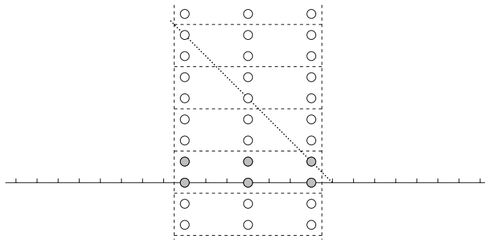
FIGURE 7. A P_{3,2}^{3,1} -tiling of level 3.
