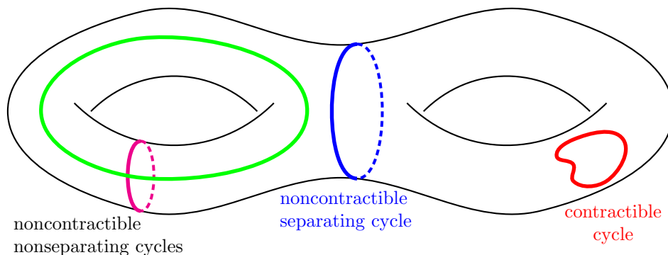
FIGURE 7. Cycles on the double torus.
