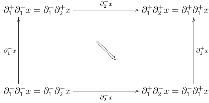
Figure 1: A 2-cube
