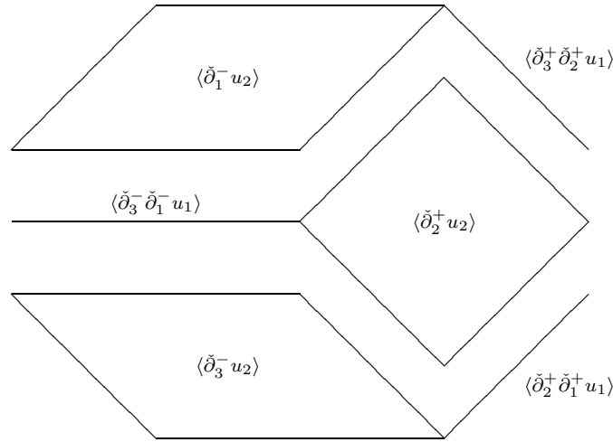
Figure 5: The decomposition of d_2^- \langle u_3 \rangle
