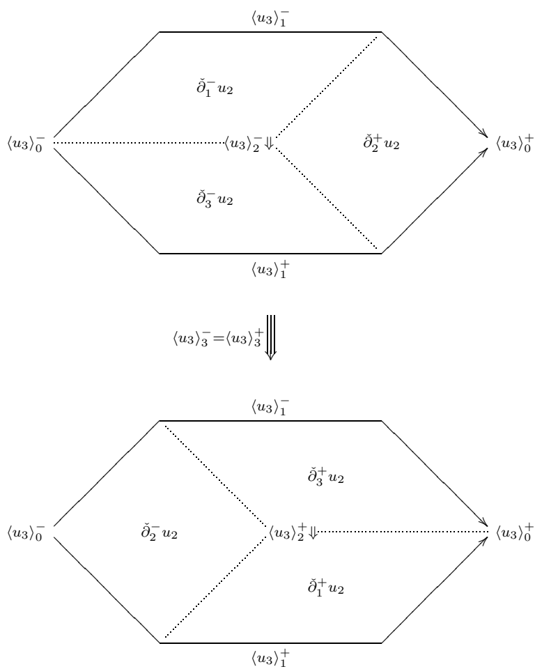
Figure 4: The chains \langle u_3 \rangle_i^\alpha
