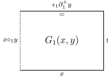
Figure 8: The composer of two 1-cubes
