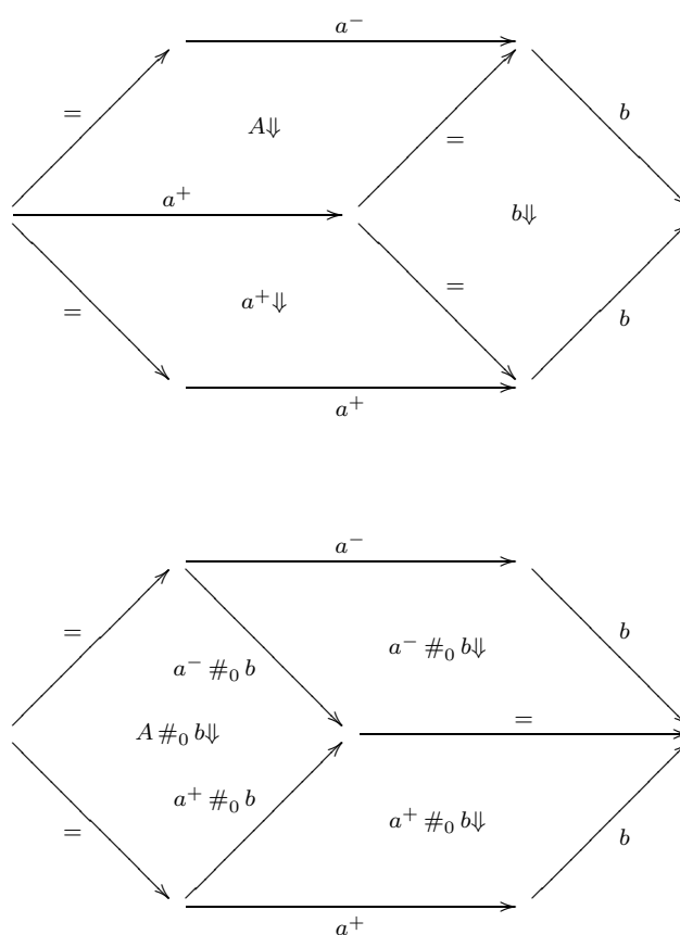
Figure 11: The shell s in the proof of Theorem 7.2
