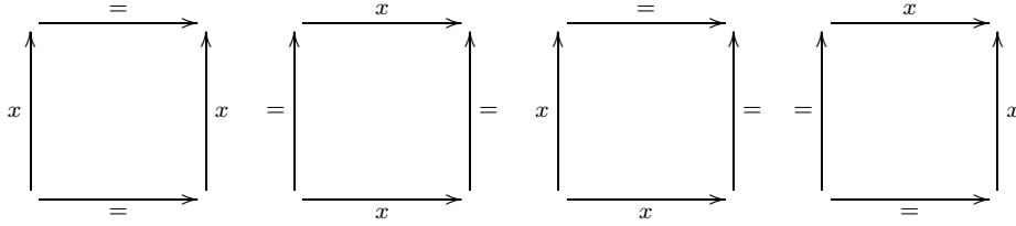
Figure 3: Admissible 2-shells
