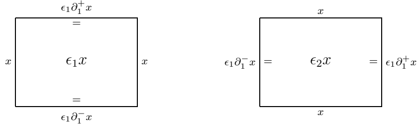
Figure 6: The degeneracies of a 1-cube
