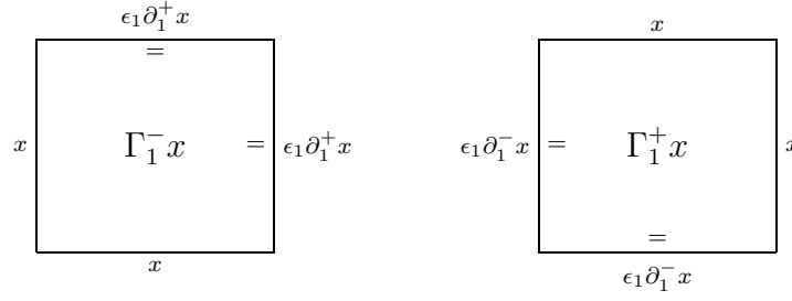
Figure 7: The connections of a 1-cube
