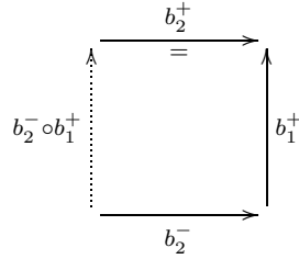
Figure 2: A 2-box opposite \partial_1^- with a unique thin filler
