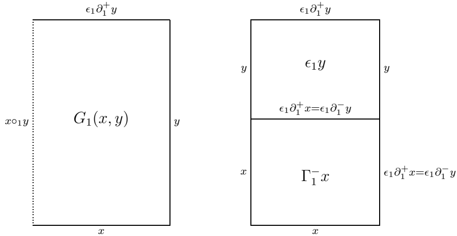
Figure 10: The equality G_1(x, y) = \Gamma_1^- x \circ_2 \epsilon_1 y
