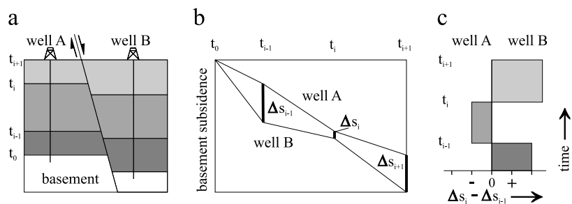
Fig. 1 Sketch illustrating the fault backstripping procedure modified from ten Veen and Kleinspehn (2000). (a) Two wells A and B on the footwall and the hanging wall of a synsedimentary normal fault, are considered. (b) Backstripping of the two wells results in basement subsidence curves. Differences in basement subsidence are expressed by \Delta s . (c) Step plot of apparent dip-slip rates vs. stratigraphic time along fault between wells A and B. Rates are calculated by subtracting \Delta s_{i-1} from \Delta s_i , and dividing the difference by the duration of the stratigraphic interval.
