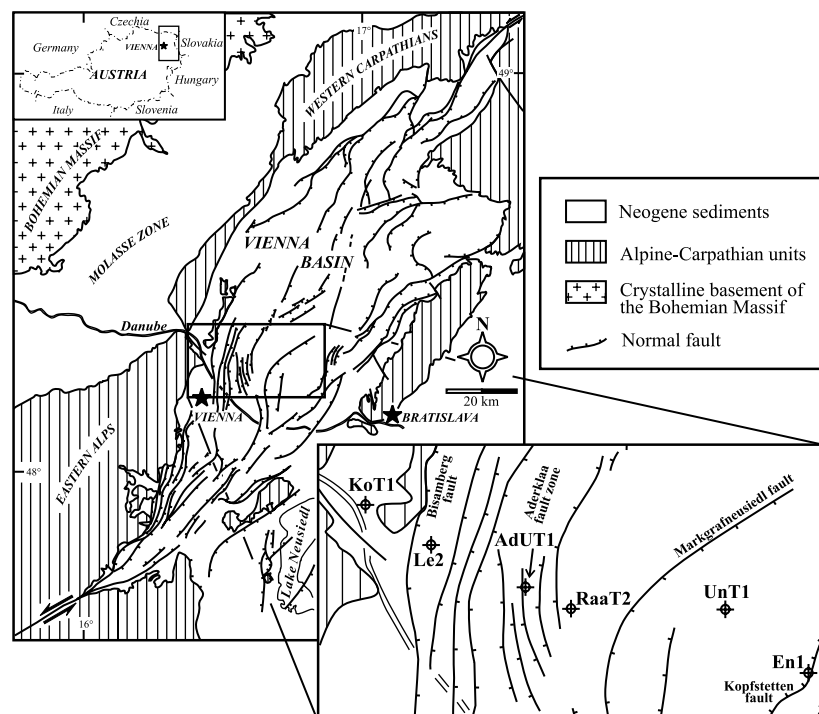
Fig. 2 Tectonic sketch map of the Vienna Basin (redrawn from Wessely, 1984; Decker, 1996) and locations of studied wells. Abbreviations: KoT1, Korneuburg T1; Le2, Leopoldau 2; AdUT1, Aderklaa UT1; RaaT2, Raasdorf T2; UnT1, Untersiebenbrunn T1; En1, Engelhartstetten 1.
