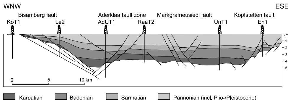
Fig. 4 WNW–ESE cross-section of the Vienna Basin along the investigated transect, based on the interpreted seismic section NV-8601/N-845D of Zych and Wessely (in Brix and Schulz, 1993). For abbreviations see Fig. 2.
