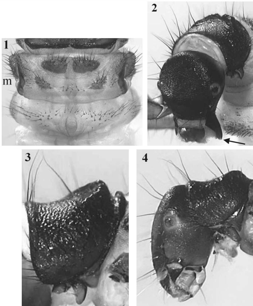
Figs 1-4. Drusus nigrescens , fifth instar larva. 1: metathorax and first abdominal segment, dorsal view (m= 6 metanotal sclerites); 2: head and pronotum, antero-lateral view; arrow: spoon-shaped mandible with straight cutting edge; 3: pronotum, left lateral view; 4: Drusus monticola , head and pronotum, left lateral view.
