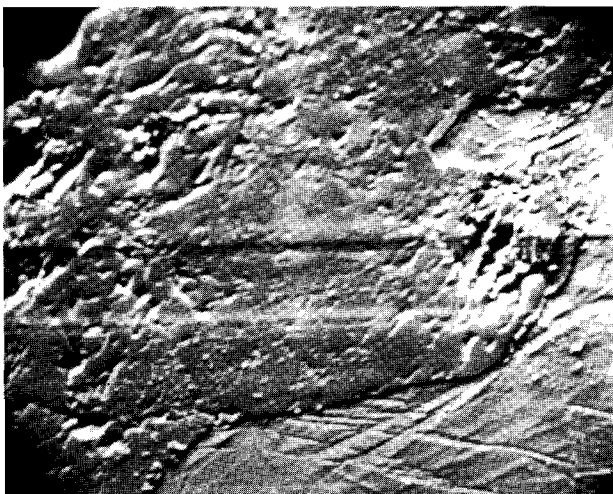
Fig. 3a. SEM picture of a chromite found at the boundary kamacite/troilite. Some elements in this unusual inclusion are shown in the other pictures. Width of the picture is 220 \mu\text{m} .
