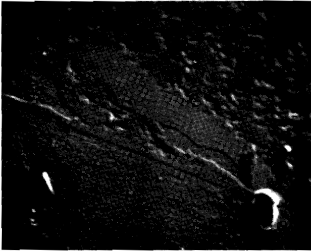
Fig. 1a. SEM-picture of one of the Ni-rich inclusions which was found at the boundary between troilite and kamacite. The object at the lower right is of artificial origin. The width of the picture is 220 \mu\text{m} . The kamacite is rimmed by rhabdite.
