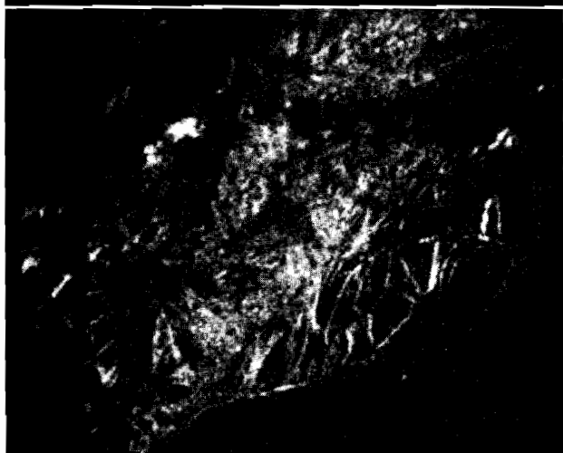
Fig. 3d. Cu-distribution picture. Copper shows a very interesting behaviour. The distribution is very inhomogenous, and the overall abundance is rather high. There is no copper visible in the troilite inclusions. Near the kamacite border a dendritic structure is visible.
