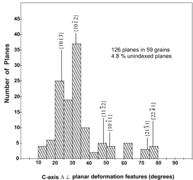
Fig. 8. A histogram of angles, binned at 5^\circ , between c-axis and poles to PDFs in quartz from suevite from drill hole BH3 at the Bosumtwi impact structure. The plot shows a strong concentration of planes at 23^\circ and 32^\circ that is characteristic for the \omega \{10\bar{1}3\} and \pi \{10\bar{1}2\} orientations respectively; 126 PDFs in 59 grains were measured; average plane/grain (P/G) ratio = 2.14 (4.76% unindexed planes).
