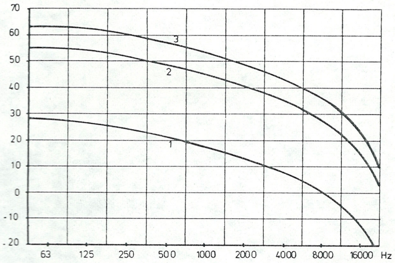
Fig. 7 Power spectrum level, expressed as sound pressure level per Hz bandwidth, of normal music-programme, performed at a maximum short-time average power level corresponding to appr. SPL 90 dB. 1. Minimum short-time average power level 2. Long-time average power level 3. Maximum short-time average power level
