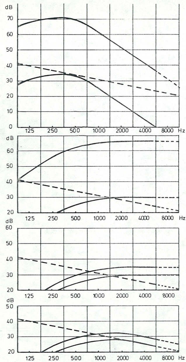
Fig. 8 Procedure for optimum transmission of speech into very noisy environment, illustrated for "pink noise threshold". — Upper and lower limiting curves for the dynamic range of speech - - - Pink noise threshold
