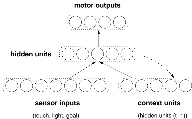
Figure 10: Meeden's recurrent neural robot control architecture. Solid arrows represent fully connected layer of weights between two layers of units (indicated by surrounding dotted lines). Hidden unit values are fed back via a weightless 1:1 copy connection (indicated by the dashed arrow) and used as extra inputs in the next time step. Adapted from (Meeden, 1996).
