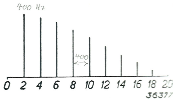
Fig. 7. Oscillogram and spectrum of two vibrations which have the same distance between the harmonics but different periodicity.
