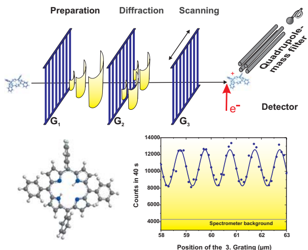
Figure 2. The wave-particle duality of the biode tetraphenylporphyrin can be revealed by diffracting the molecules in a near-field interferometer of the Talbot–Lau type (Hackermüller et al. , 2003). Molecules passing the first grating are diffracted and delocalized over several micrometers at the second grating. Diffraction there leads to interference fringes, i.e., a molecular density pattern, at the position of the third mask. This is imaged by scanning grating G 3 and by recording all transmitted molecules in a mass spectrometer.
